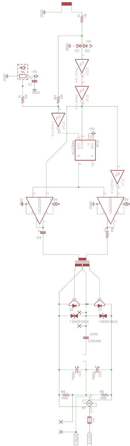
Figure 5: Driver and Bridge Circuit Schematic, from oneTesla's webpage
